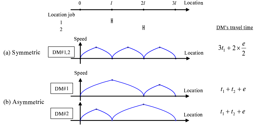
Fig. 3. Example of non-optimal symmetric schedule (in acceleration-constrained case): Two location jobs have zero-length feasible location intervals with execution time e .
