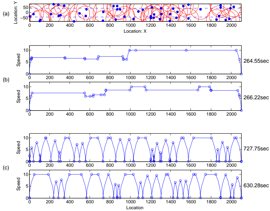
Fig. 6. Example of speed control plans (50 nodes, Number of data mules k = 2 ): (a) Node placement. Filled circles are the node locations and large circles represent communication ranges. Two dotted lines correspond to the trajectories of two data mules; (b) Speed control plans from the heuristic algorithms; (c) Speed control plans from the naive method.
