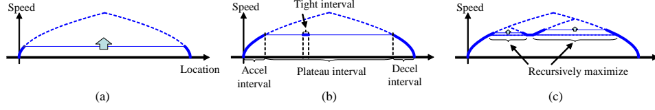
Fig. 2. Idea of the heuristic algorithm: (a) Increase the plateau speed. Dotted curves show the acceleration / deceleration for the fastest possible travel covering the whole interval. Bold and thin lines mean fixed intervals and free intervals, respectively. (b) A tight interval is found. (c) Recursively maximize the speed for the remaining free intervals.
