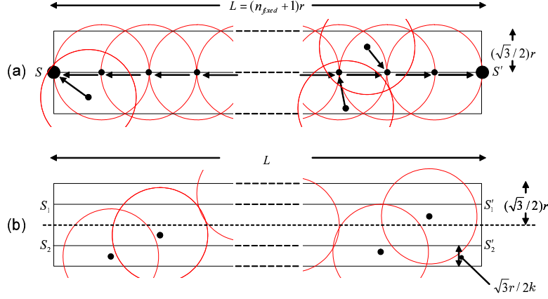
Fig. 5. Randomly generating test cases: (a) For comparison with multihop forwarding. Fixed nodes are aligned on line SS' ; (b) For multiple data mules case. An example with two data mules ( k = 2 ) is shown.
