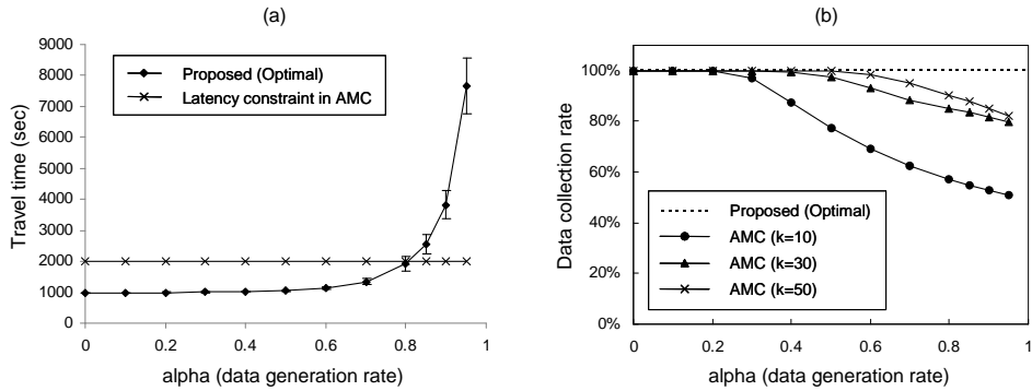
Fig. 9. Comparison with Adaptive Motion Control (AMC): Sparse deployment ( L = 2000 )
